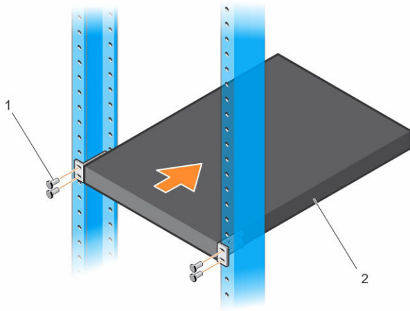
Figure 7. Mounting N20xx in 2-Post Rack
