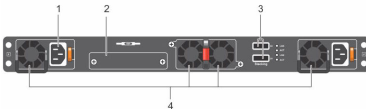
Figure 12. N30xx PSU-Side
