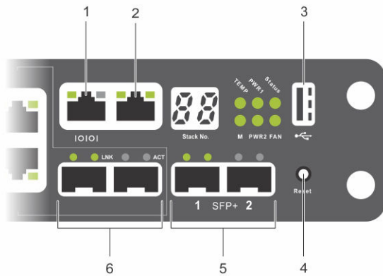
Figure 11. N30xx Close-up
