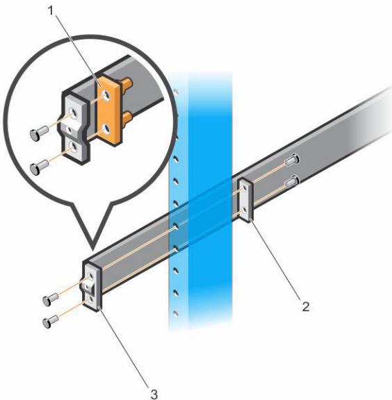
Figure 15. 2-Post Flush-Mount Configuration
